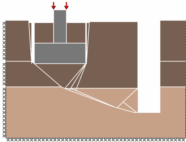
Figure 5: Failure mechanism for the problem after trench excavation
