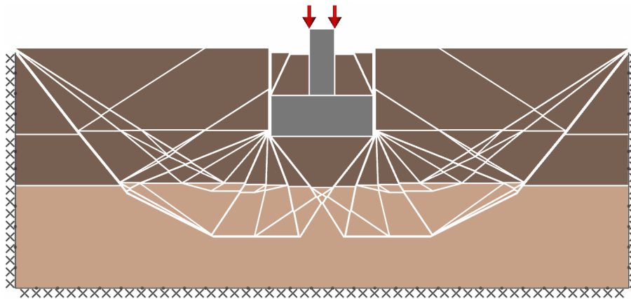
Figure 3: Main problem restrained failure mode
