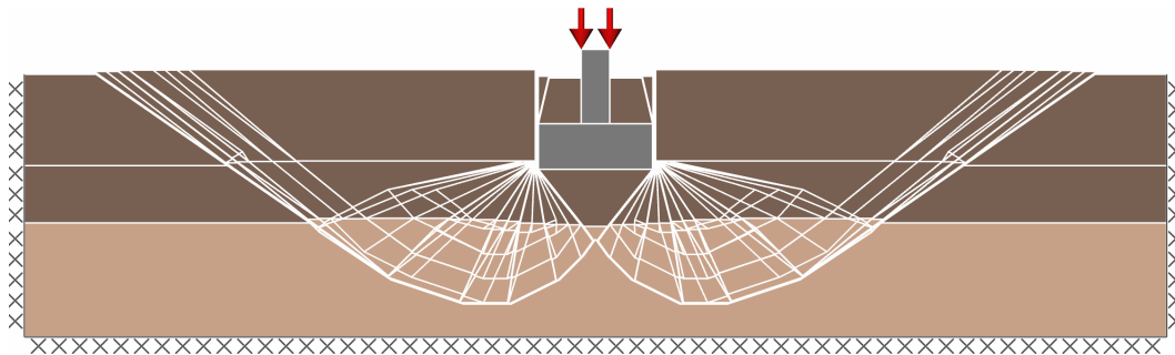
Figure 4: Main problem failure mode
