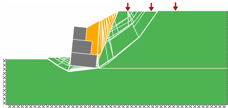
Figure 1: Global failure mechanism for analysed problem
